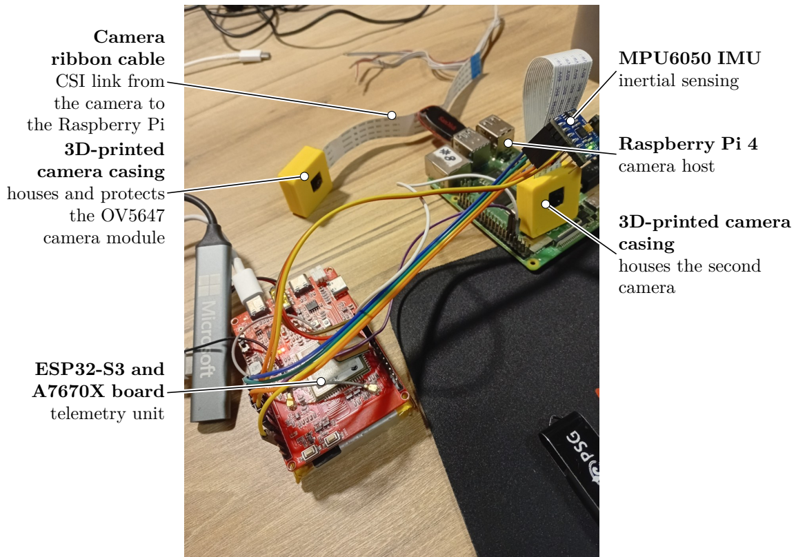
Figure 3.5: The cameras fitted in their 3D-printed casings, shown with the rest of the bench setup.
